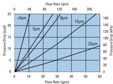
W322 8" DT Filter Only DT-9800-8, 8"/203mm
