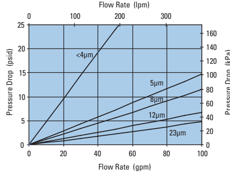
W621 8" DX2 Filter Only DX2-9600-8, 8.23"/209mm
