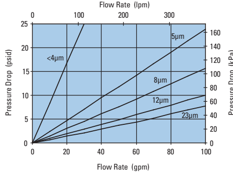
W621 13" DT Filter Only DT-9600-13, 12.913"/327.8mm
